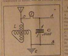
Showing the Variometer and Condenser Adjustment.
